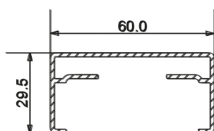
■ MAIN COURANTE GC4006N
