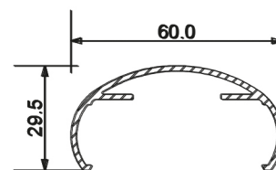
● MAIN COURANTE GC4002
